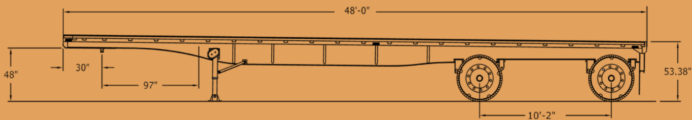
MODEL: FC - 48
