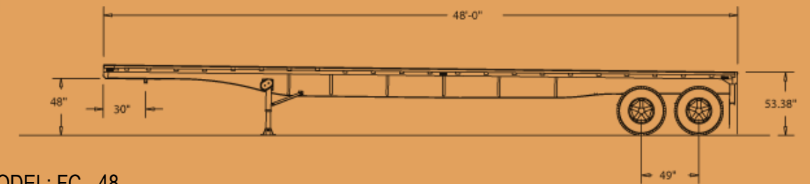
MODEL: FC - 48
